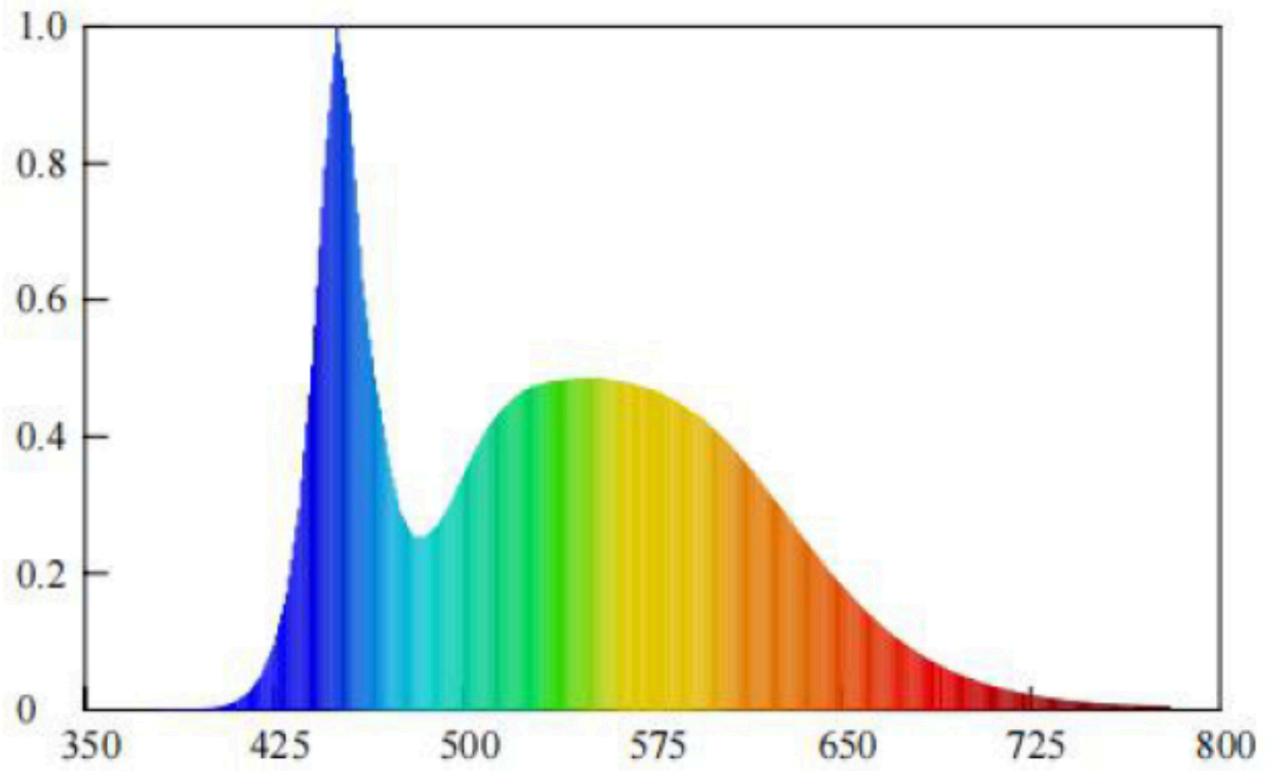
Spectral power distribution (6500K)
